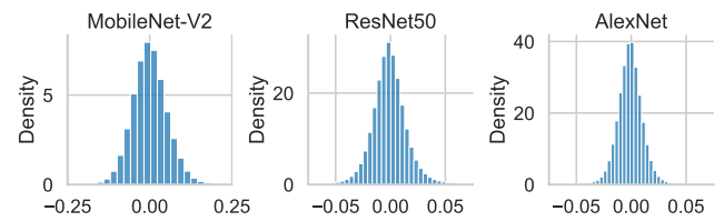
Fig. 3: Distribution of Pretrained Weights for Various Models
