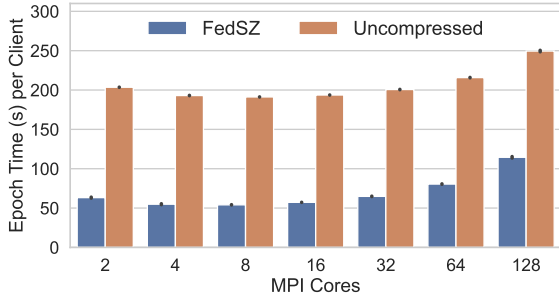
(a) Weak Scaling Results
