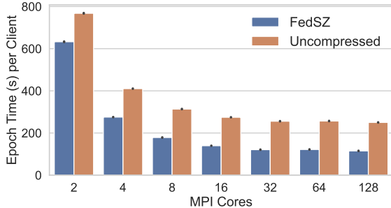
(b) Strong Scaling Results
